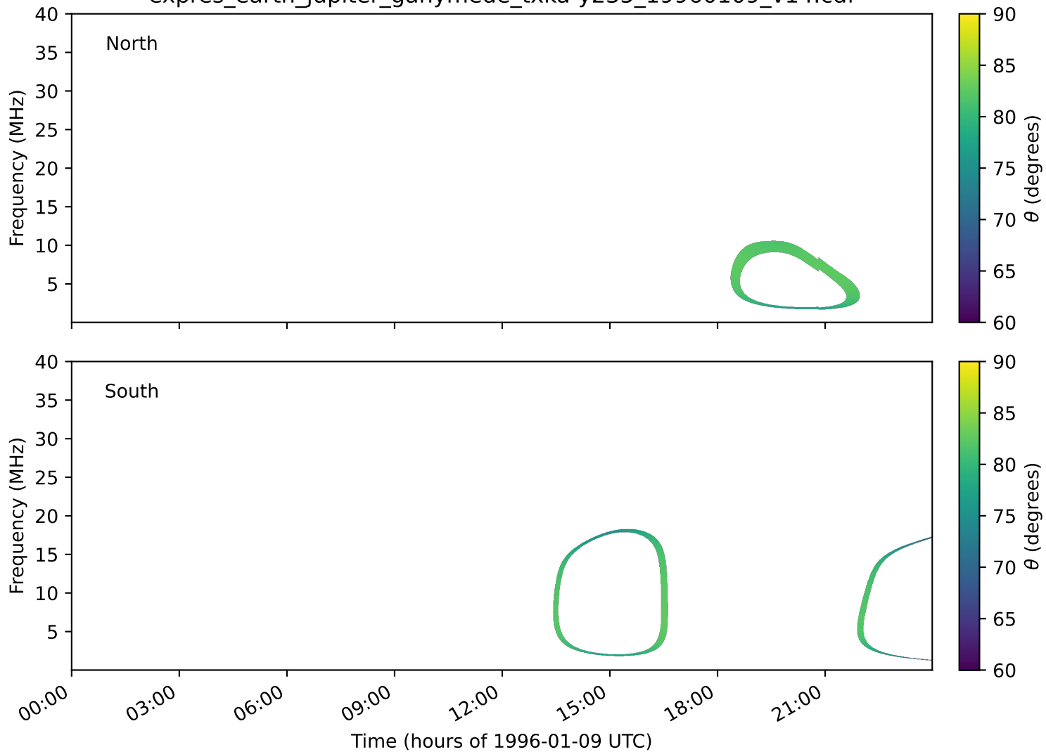
expres_earth_jupiter_ganymede_txka-y235_19960109_v14.cdf
