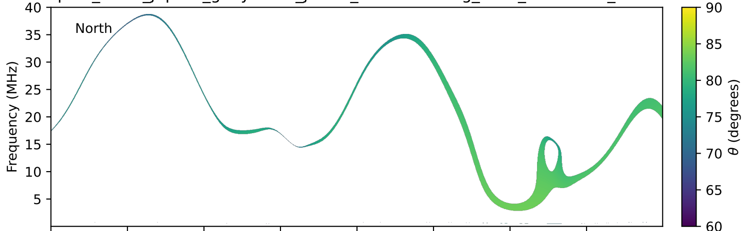
expres_earth_jupiter_ganymede_jrm33_lossc-wid1deg_3kev_19960120_v11.cdf
