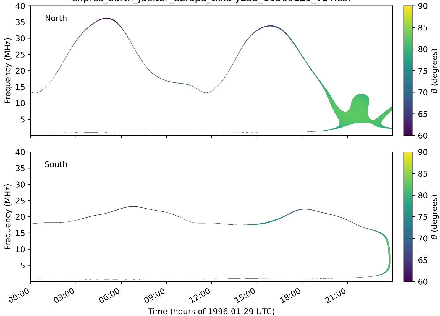
expres_earth_jupiter_europa_txka-y235_19960129_v14.cdf
