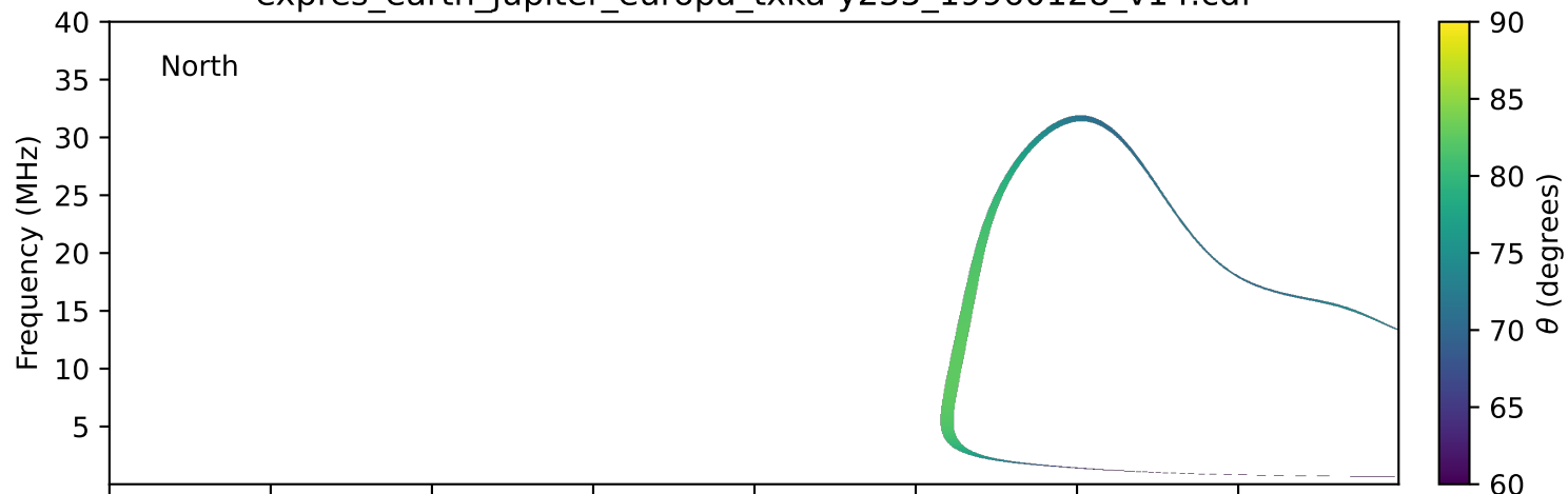
expres_earth_jupiter_europa_txka-y235_19960128_v14.cdf
