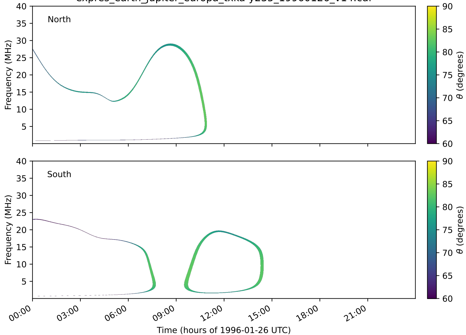
expres_earth_jupiter_europa_txka-y235_19960126_v14.cdf
