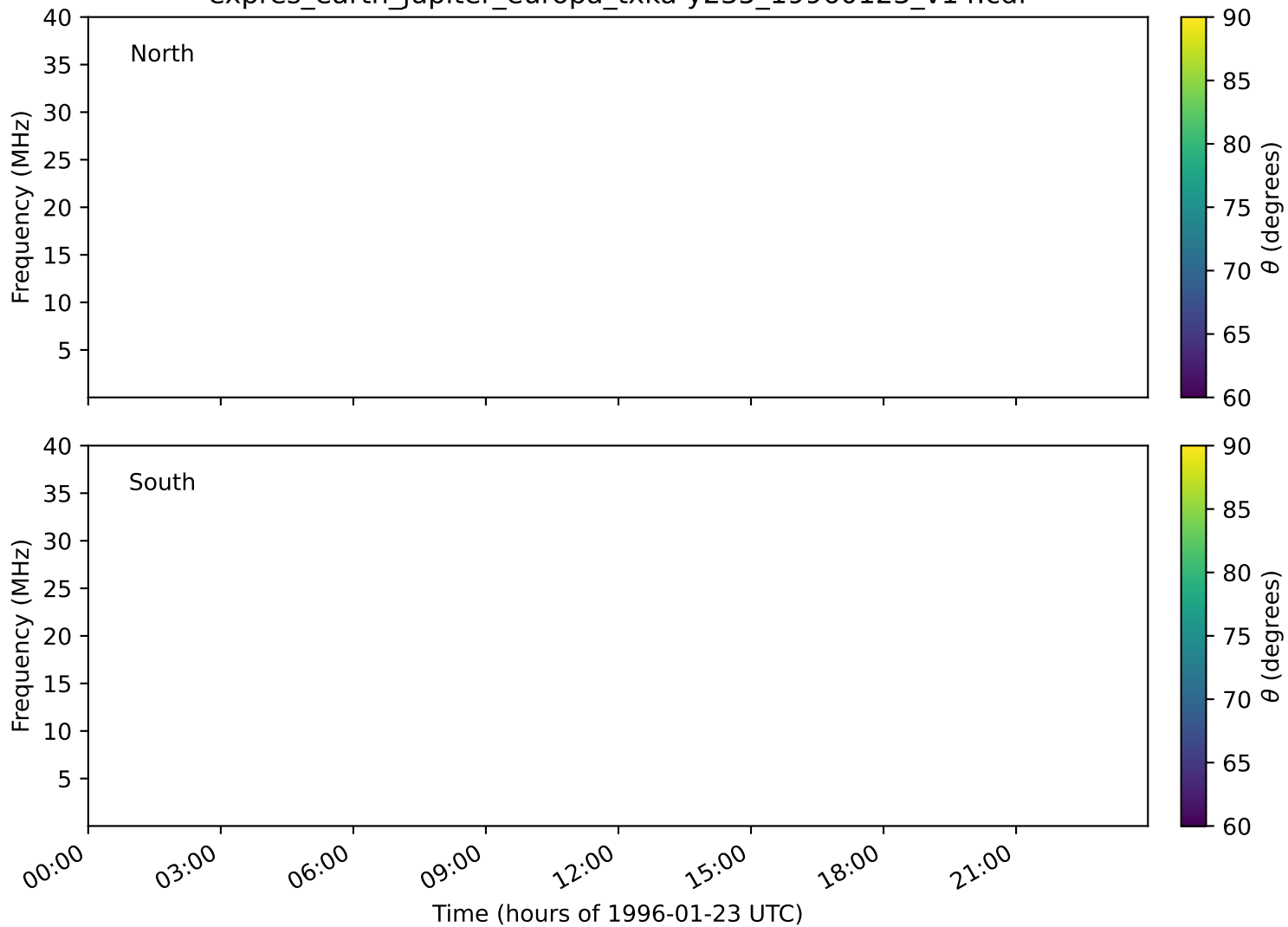
expres_earth_jupiter_europa_txka-y235_19960123_v14.cdf
