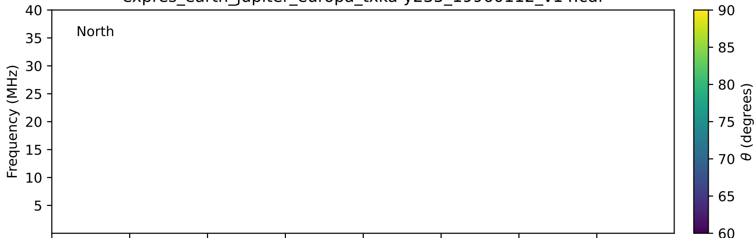
expres_earth_jupiter_europa_txka-y235_19960112_v14.cdf
