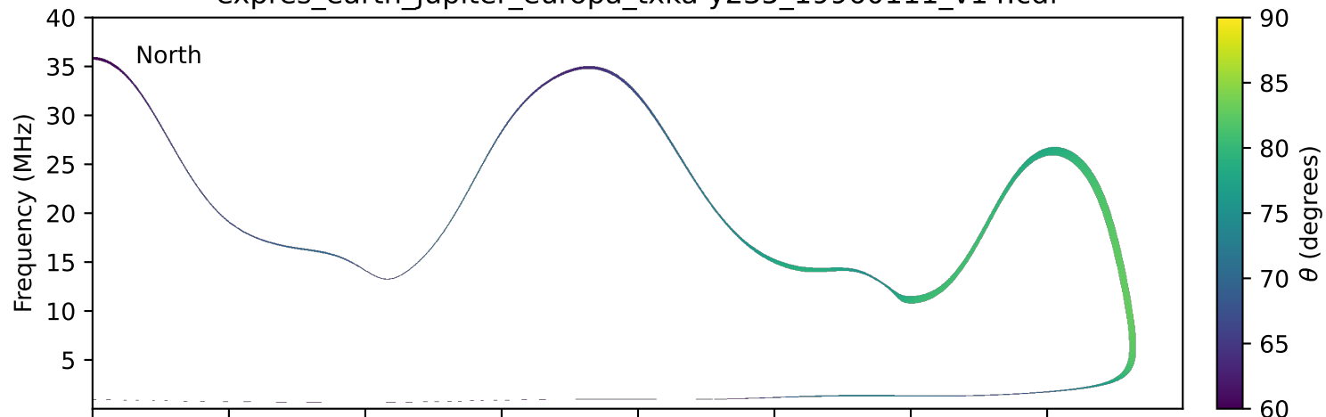
expres_earth_jupiter_europa_txka-y235_19960111_v14.cdf
