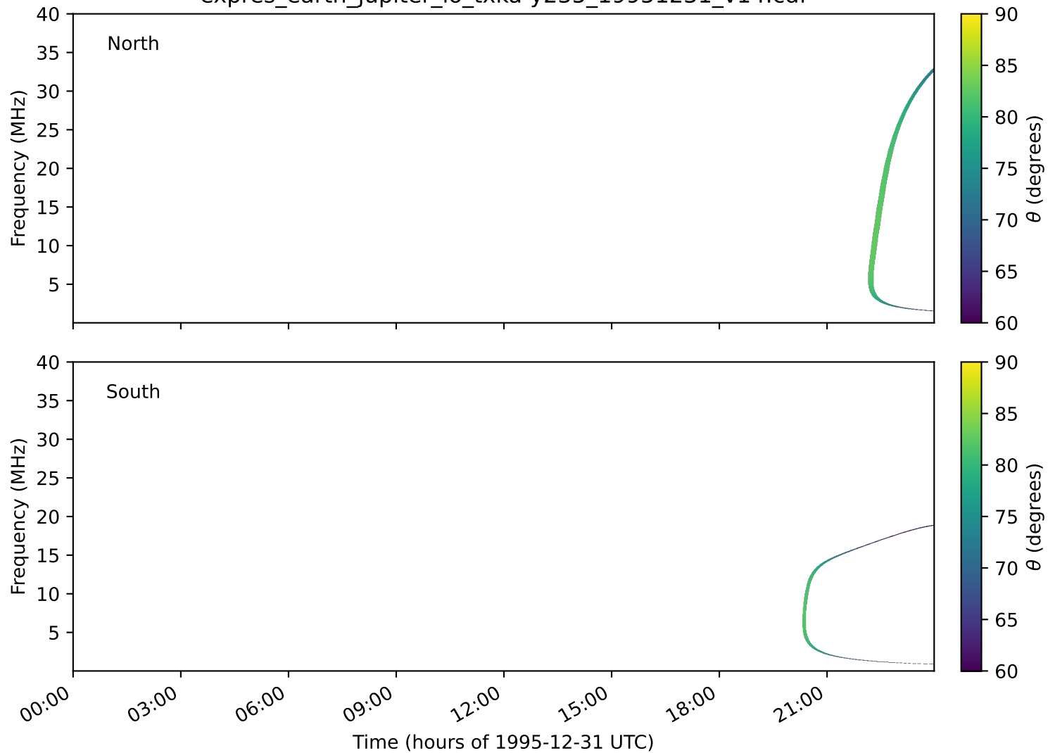
expres_earth_jupiter_io_txka-y235_19951231_v14.cdf
