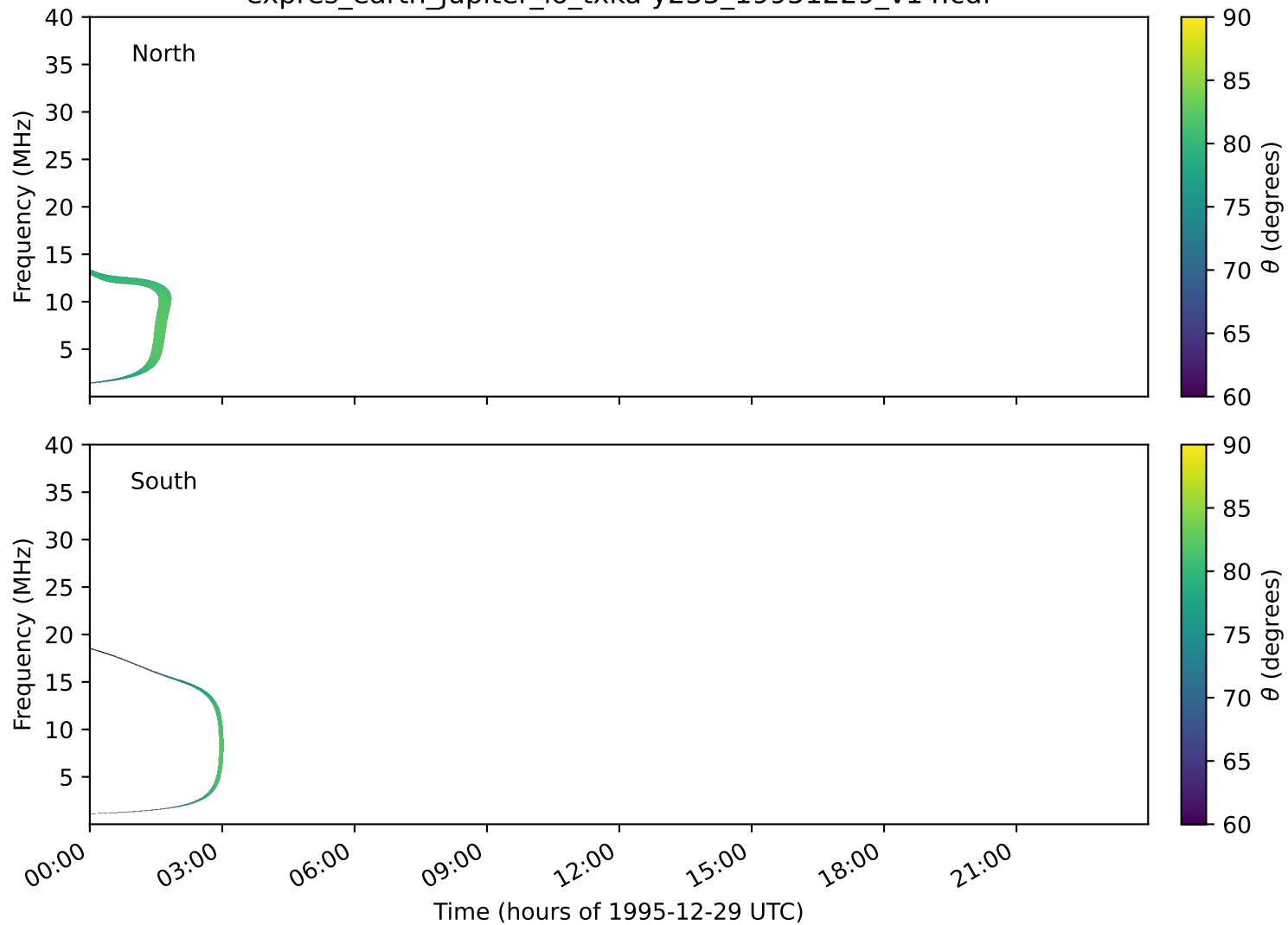
expres_earth_jupiter_io_txka-y235_19951229_v14.cdf
