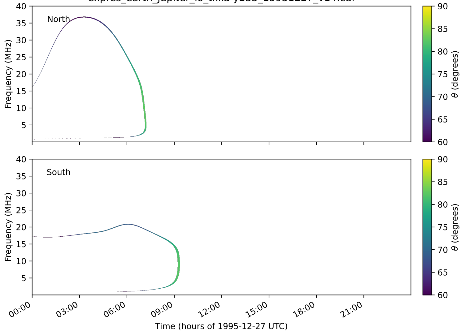
expres_earth_jupiter_io_txka-y235_19951227_v14.cdf
