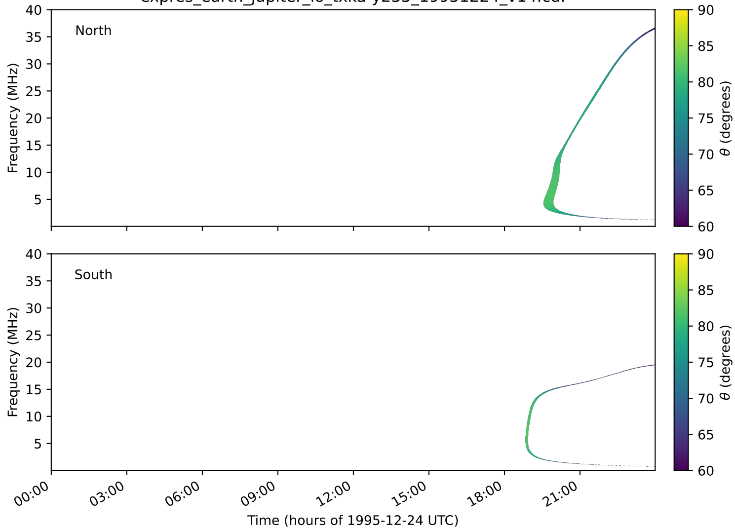
expres_earth_jupiter_io_txka-y235_19951224_v14.cdf
