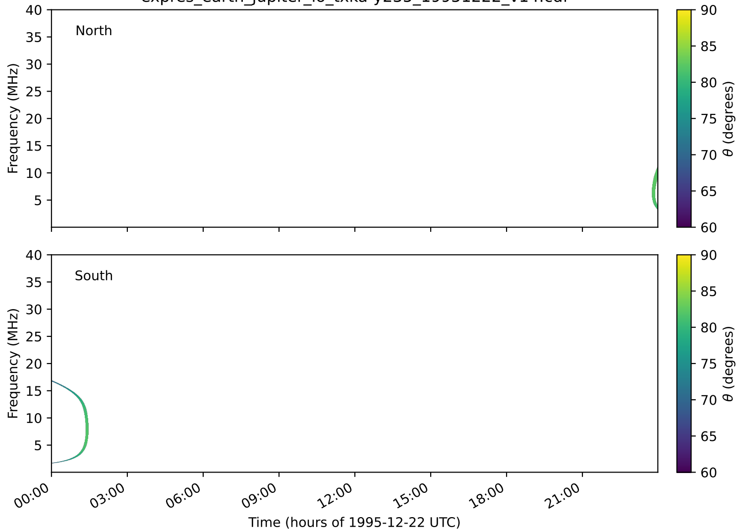
expres_earth_jupiter_io_txka-y235_19951222_v14.cdf
