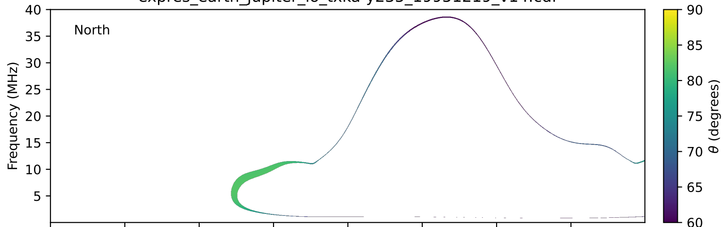
expres_earth_jupiter_io_txka-y235_19951219_v14.cdf
