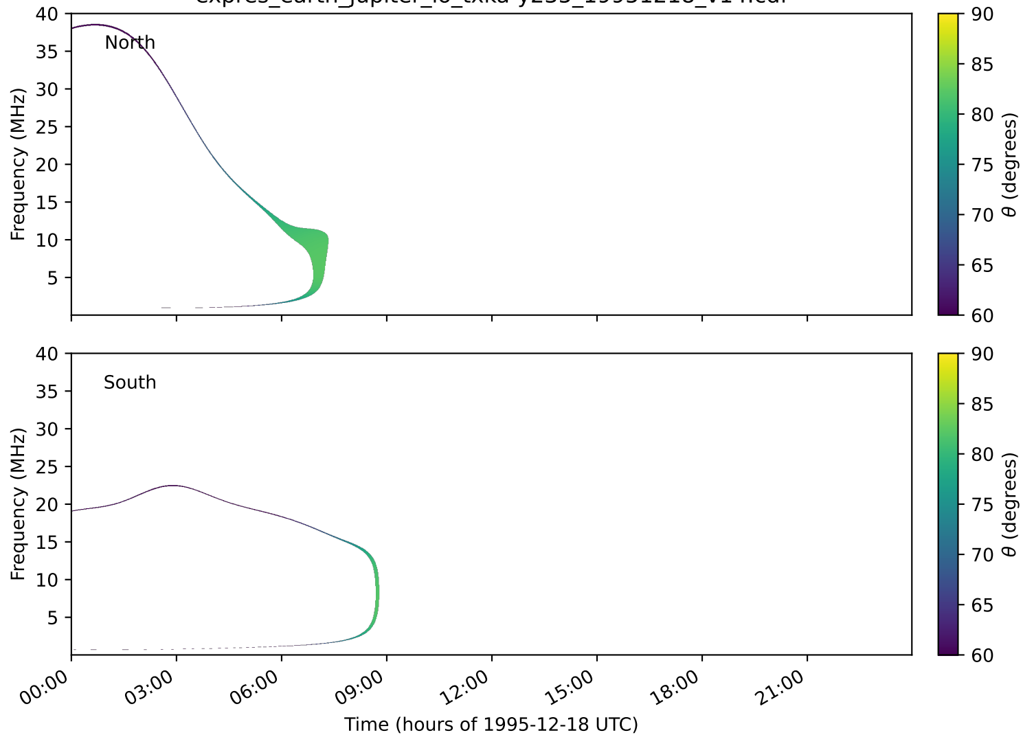
expres_earth_jupiter_io_txka-y235_19951218_v14.cdf
