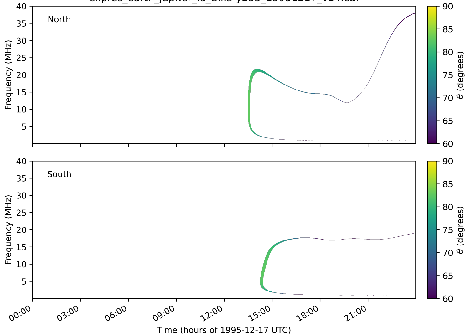
expres_earth_jupiter_io_txka-y235_19951217_v14.cdf
