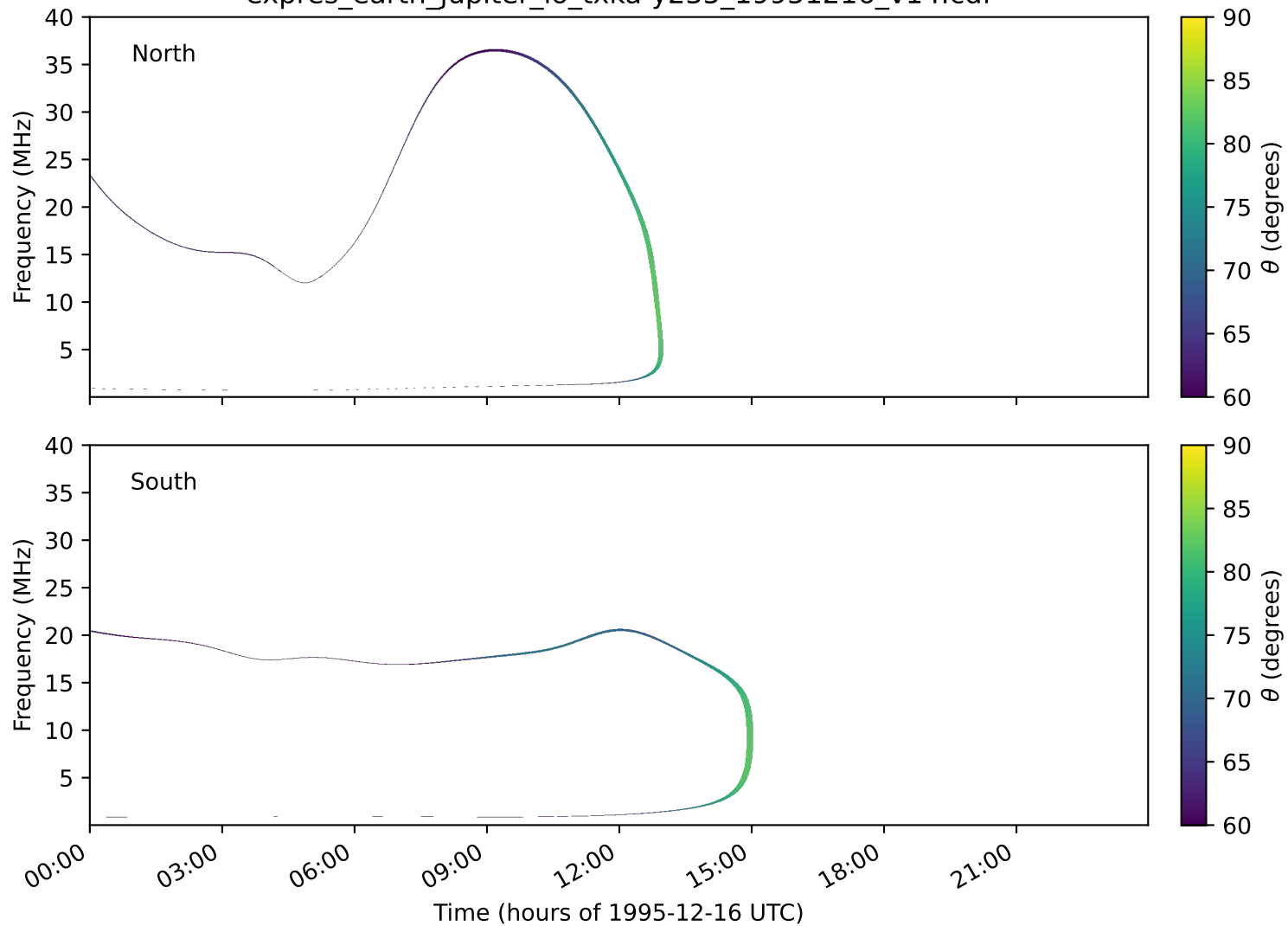
expres_earth_jupiter_io_txka-y235_19951216_v14.cdf
