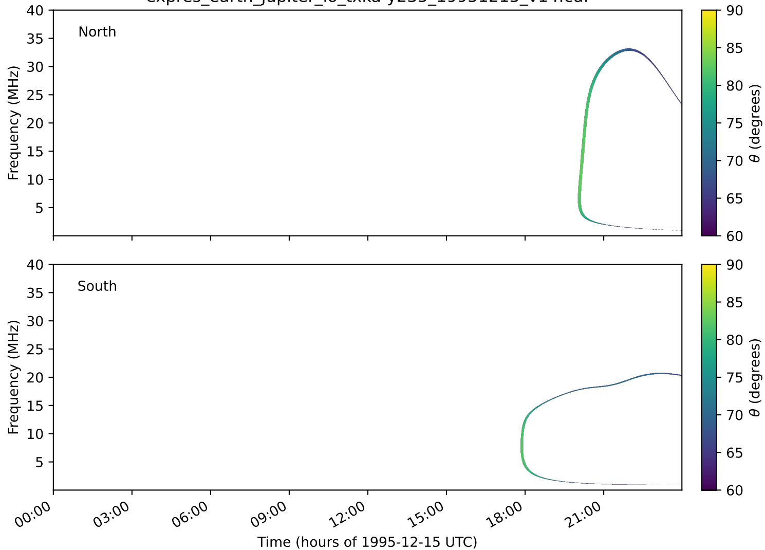
expres_earth_jupiter_io_txka-y235_19951215_v14.cdf
