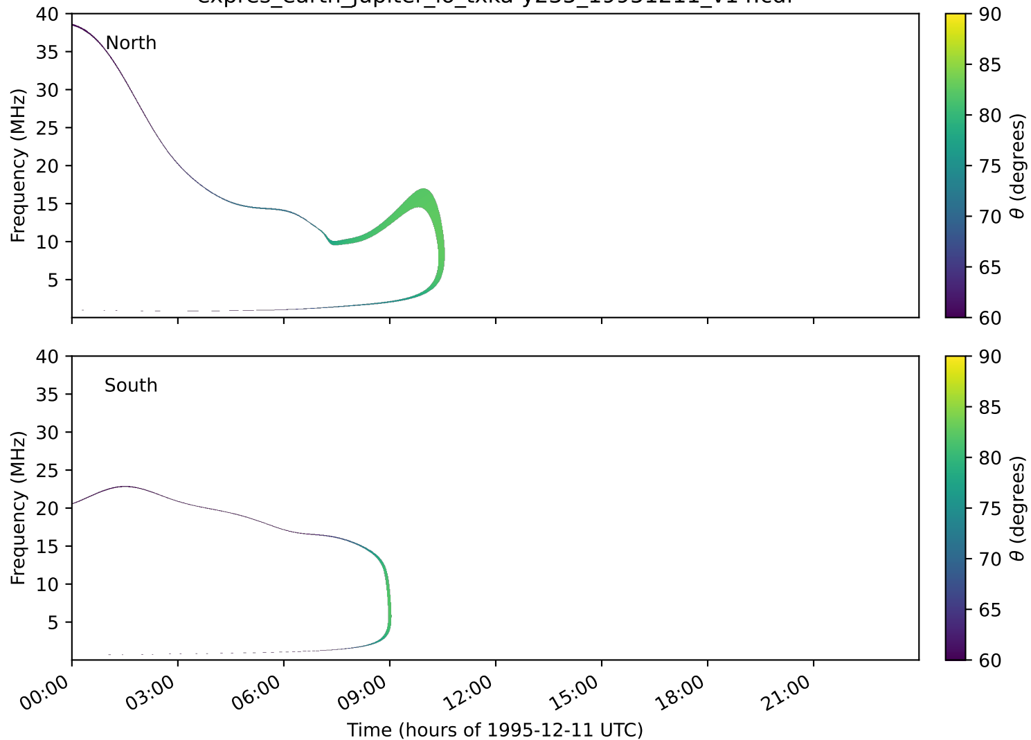
expres_earth_jupiter_io_txka-y235_19951211_v14.cdf
