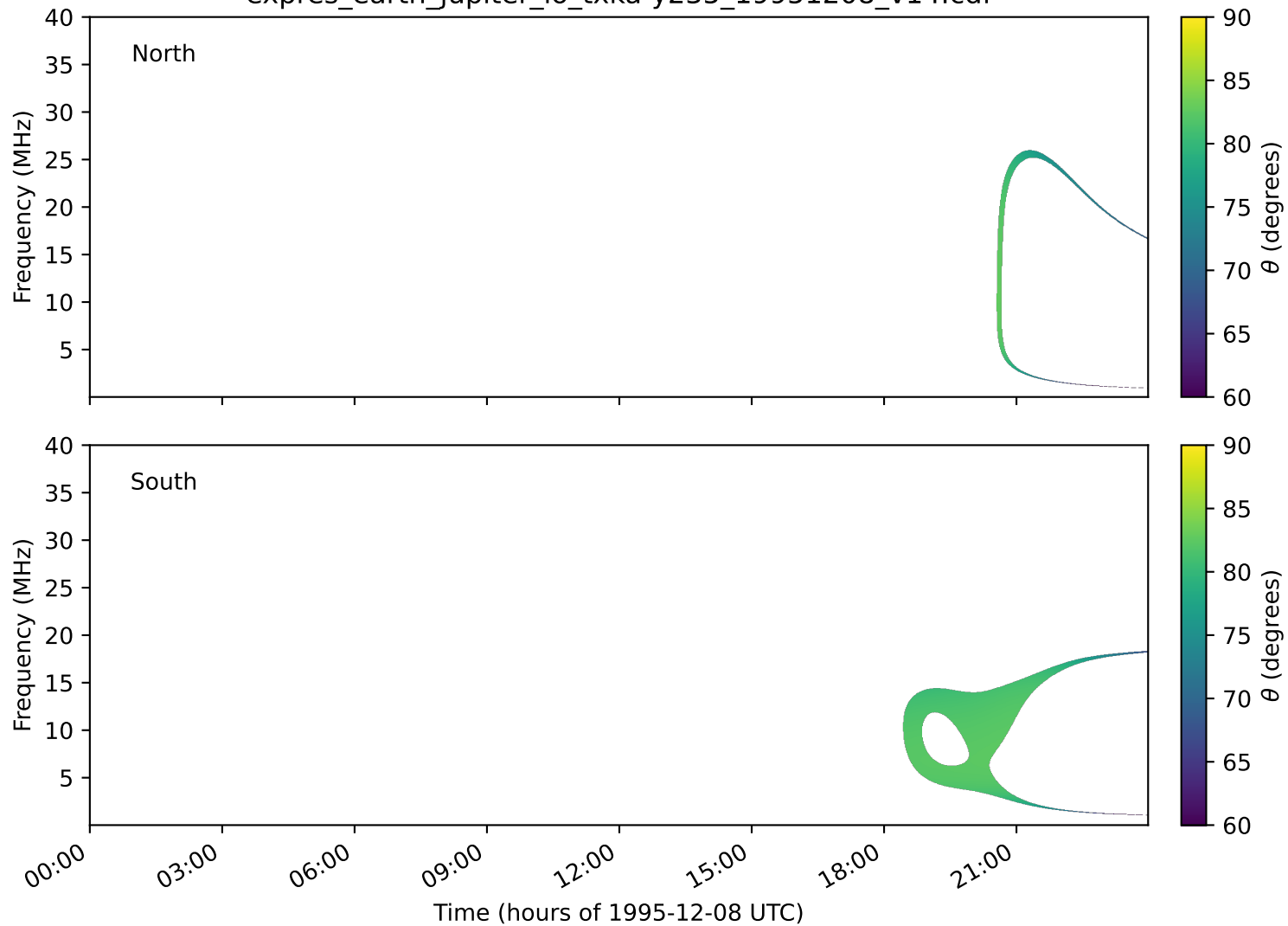
expres_earth_jupiter_io_txka-y235_19951208_v14.cdf
