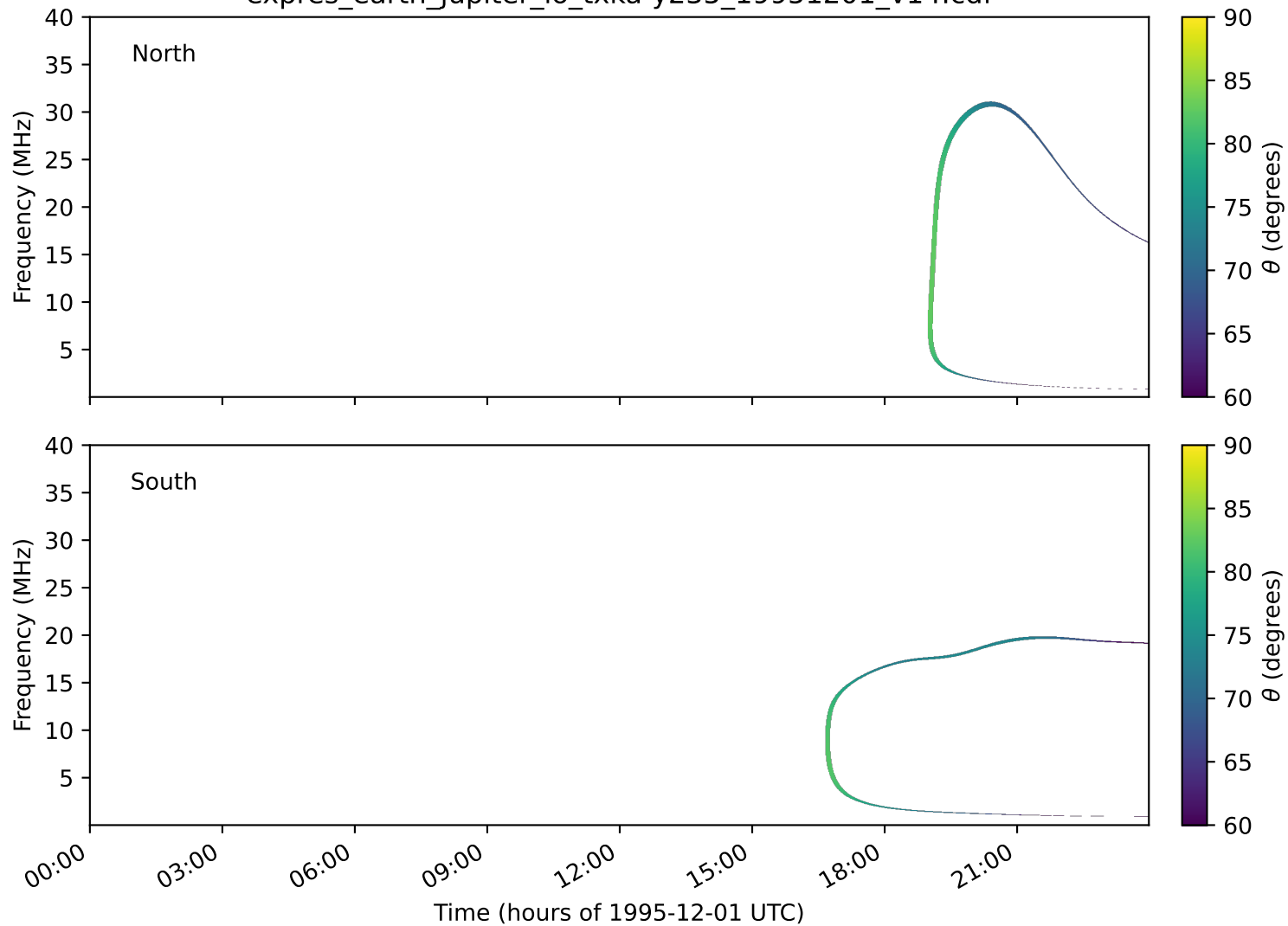
expres_earth_jupiter_io_txka-y235_19951201_v14.cdf
