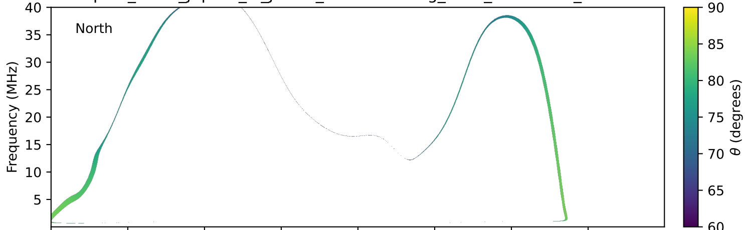
expres_earth_jupiter_io_jrm33_lossc-wid1deg_3kev_19951214_v11.cdf
