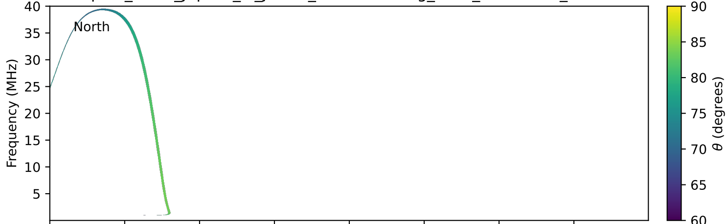
expres_earth_jupiter_io_jrm33_lossc-wid1deg_3kev_19951213_v11.cdf
