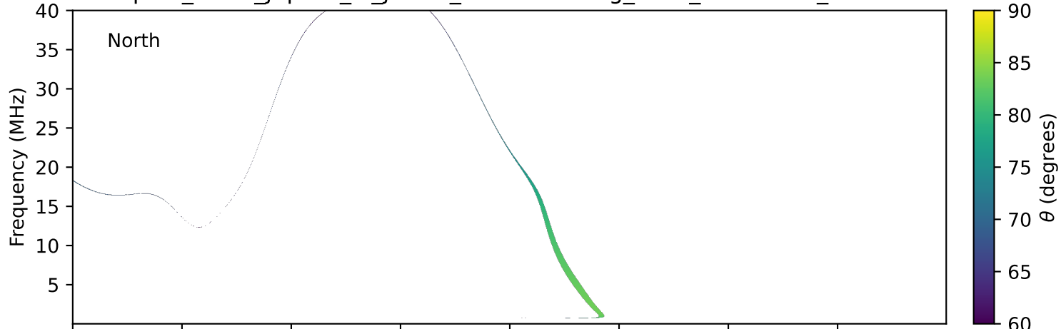
expres_earth_jupiter_io_jrm33_lossc-wid1deg_3kev_19951209_v11.cdf
