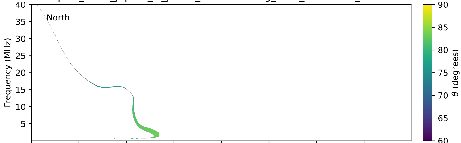
expres_earth_jupiter_io_jrm33_lossc-wid1deg_3kev_19951204_v11.cdf
