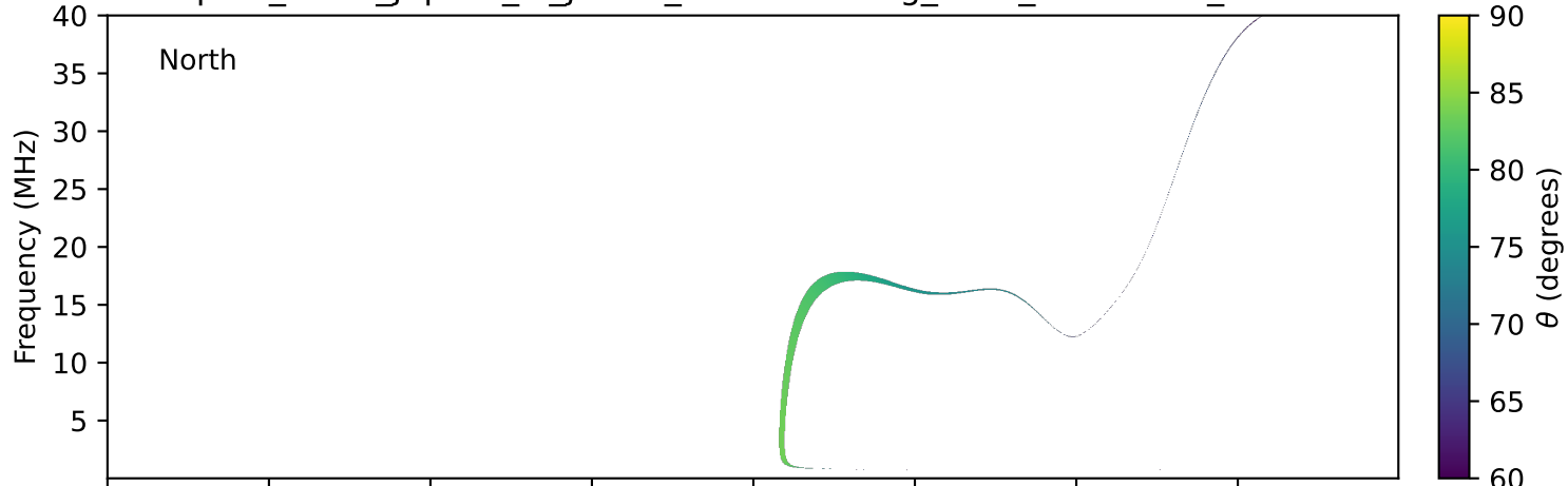
expres_earth_jupiter_io_jrm33_lossc-wid1deg_3kev_19951203_v11.cdf
