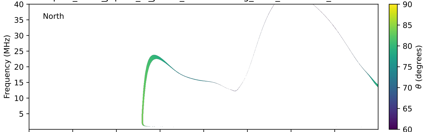
expres_earth_jupiter_io_jrm09_lossc-wid1deg_3kev_19951228_v11.cdf
