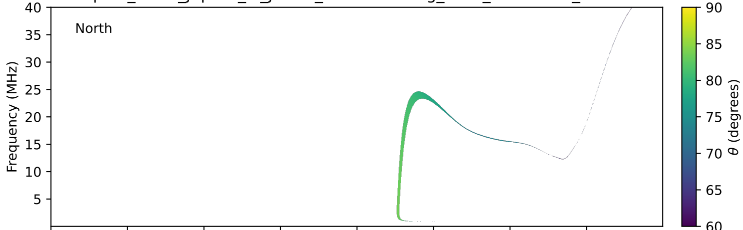
expres_earth_jupiter_io_jrm09_lossc-wid1deg_3kev_19951217_v11.cdf
