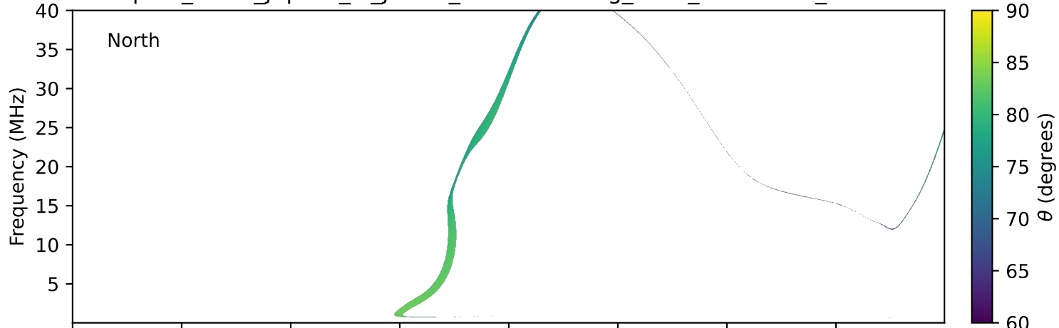
expres_earth_jupiter_io_jrm09_lossc-wid1deg_3kev_19951212_v11.cdf
