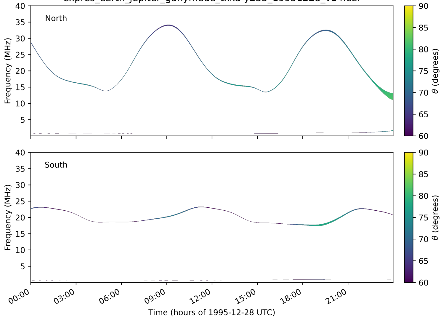
expres_earth_jupiter_ganymede_txka-y235_19951228_v14.cdf
