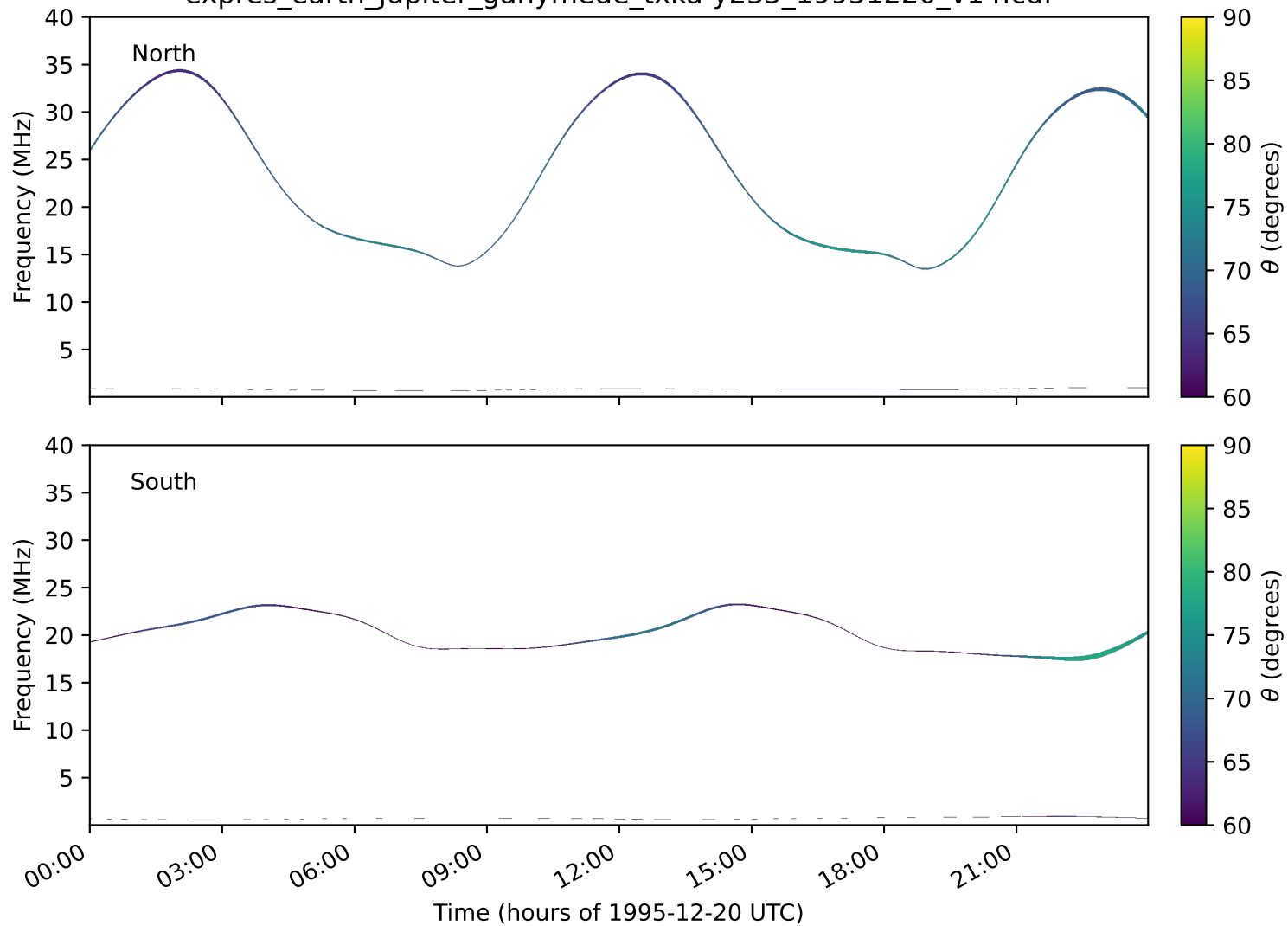
expres_earth_jupiter_ganymede_txka-y235_19951220_v14.cdf
