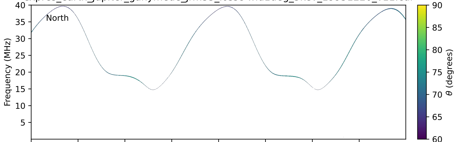
expres_earth_jupiter_ganymede_jrm33_lossc-wid1deg_3kev_19951220_v11.cdf
