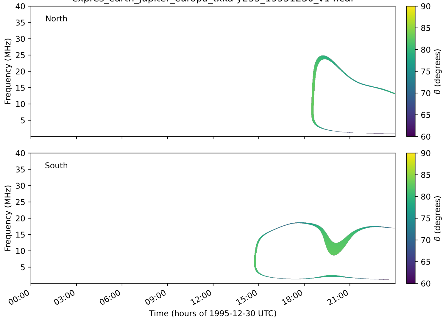
expres_earth_jupiter_europa_txka-y235_19951230_v14.cdf
