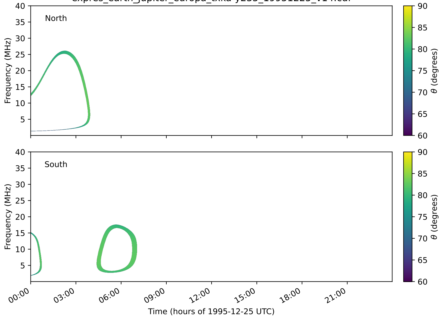
expres_earth_jupiter_europa_txka-y235_19951225_v14.cdf
