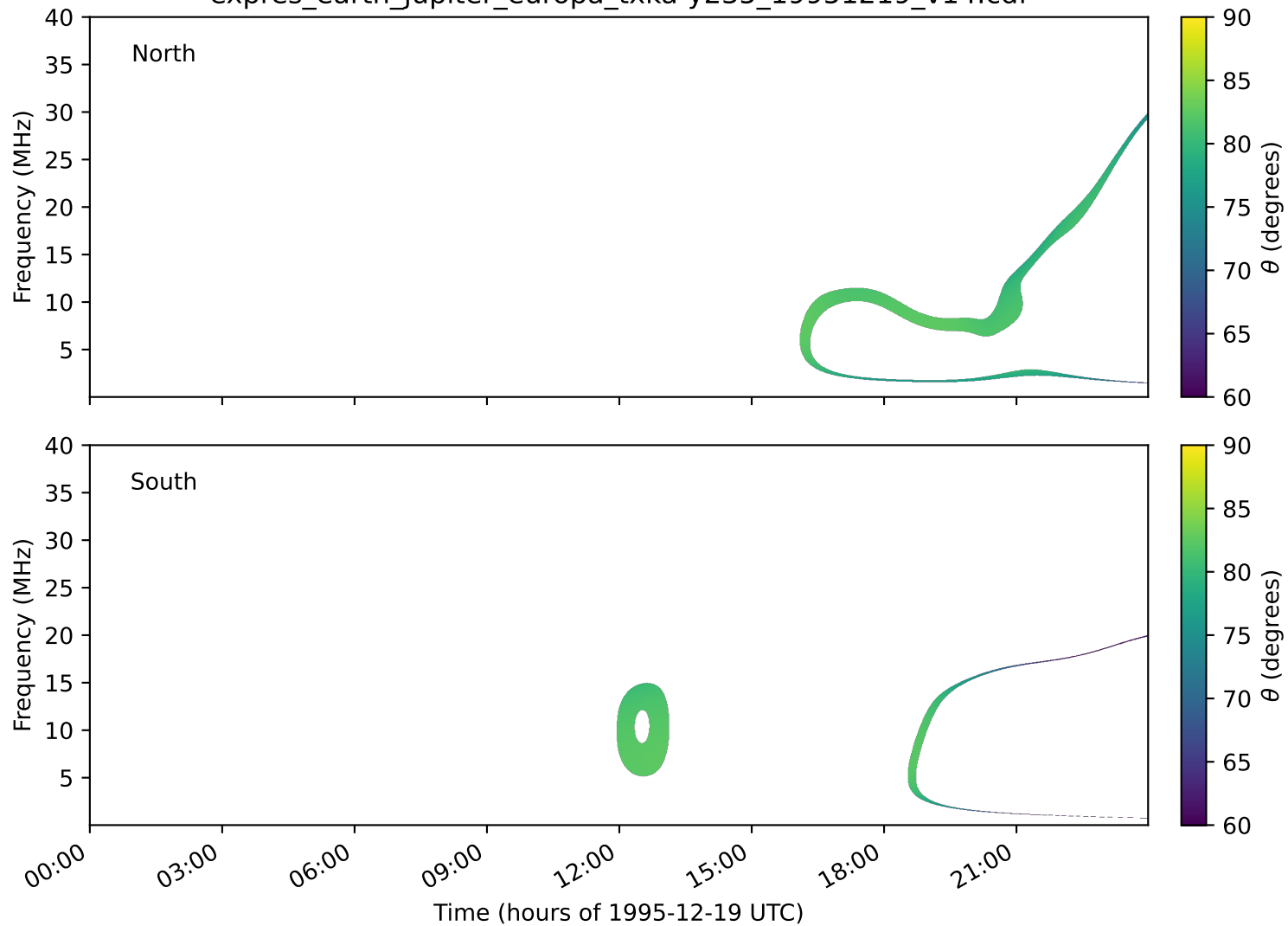
expres_earth_jupiter_europa_txka-y235_19951219_v14.cdf
