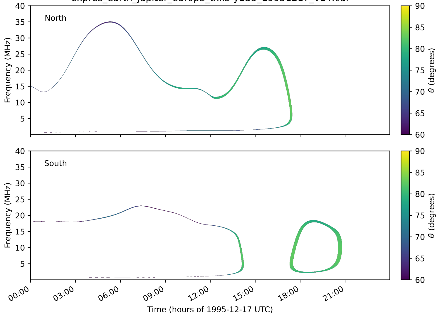
expres_earth_jupiter_europa_txka-y235_19951217_v14.cdf
