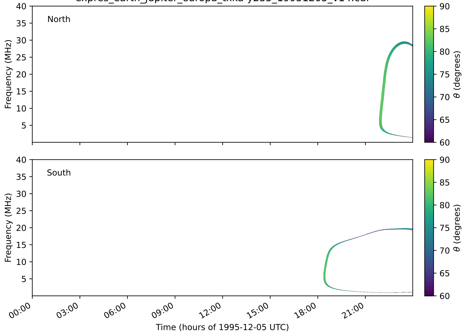
expres_earth_jupiter_europa_txka-y235_19951205_v14.cdf
