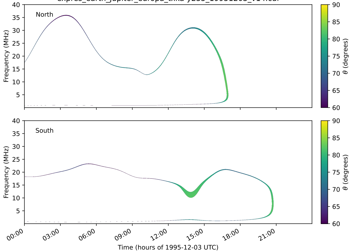
expres_earth_jupiter_europa_txka-y235_19951203_v14.cdf
