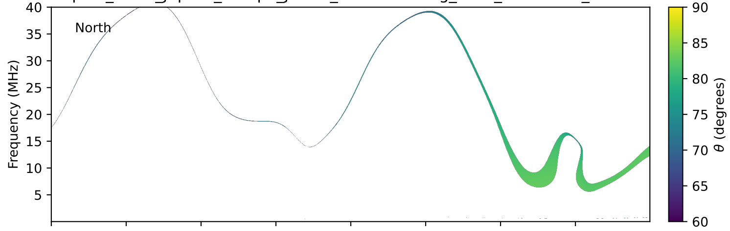
expres_earth_jupiter_europa_jrm33_lossc-wid1deg_3kev_19951210_v11.cdf
