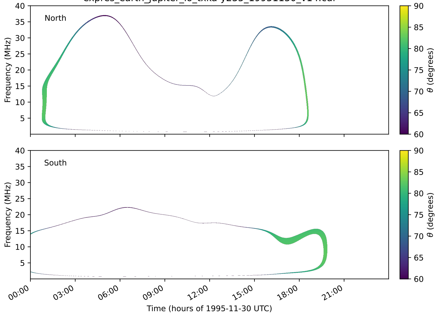
expres_earth_jupiter_io_txka-y235_19951130_v14.cdf
