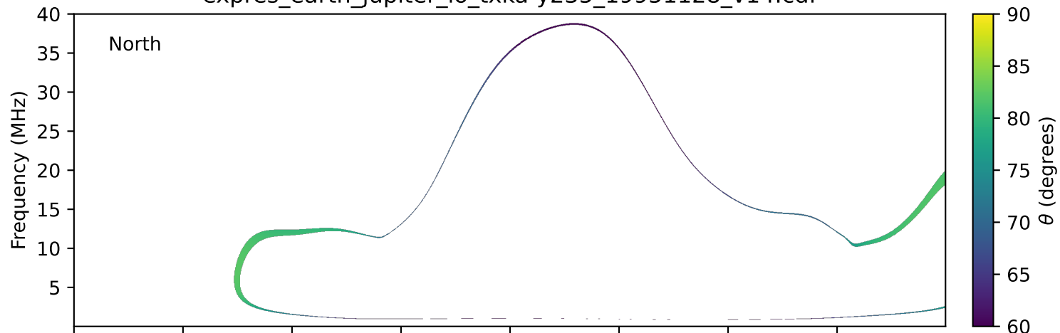
expres_earth_jupiter_io_txka-y235_19951128_v14.cdf
