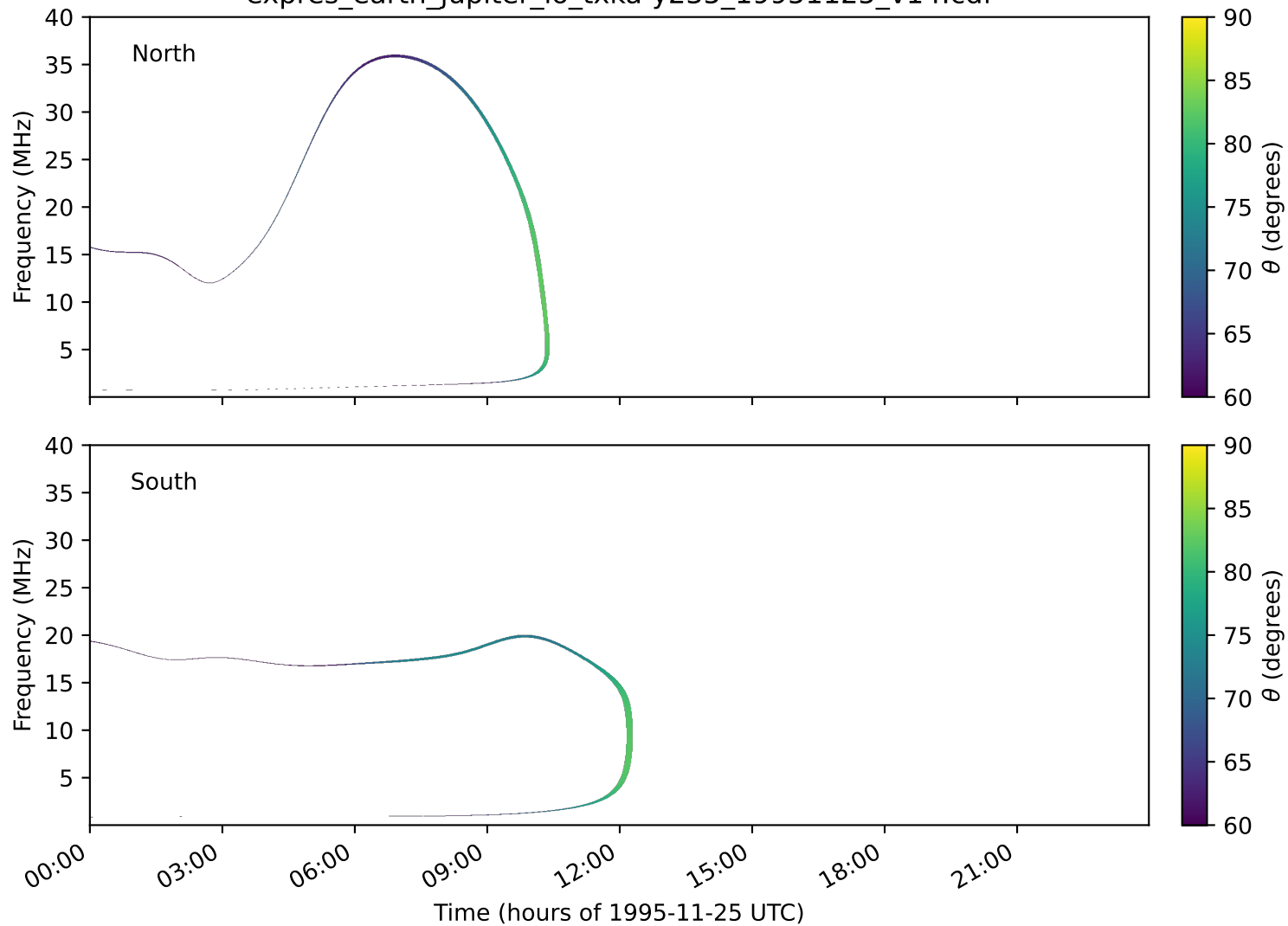
expres_earth_jupiter_io_txka-y235_19951125_v14.cdf
