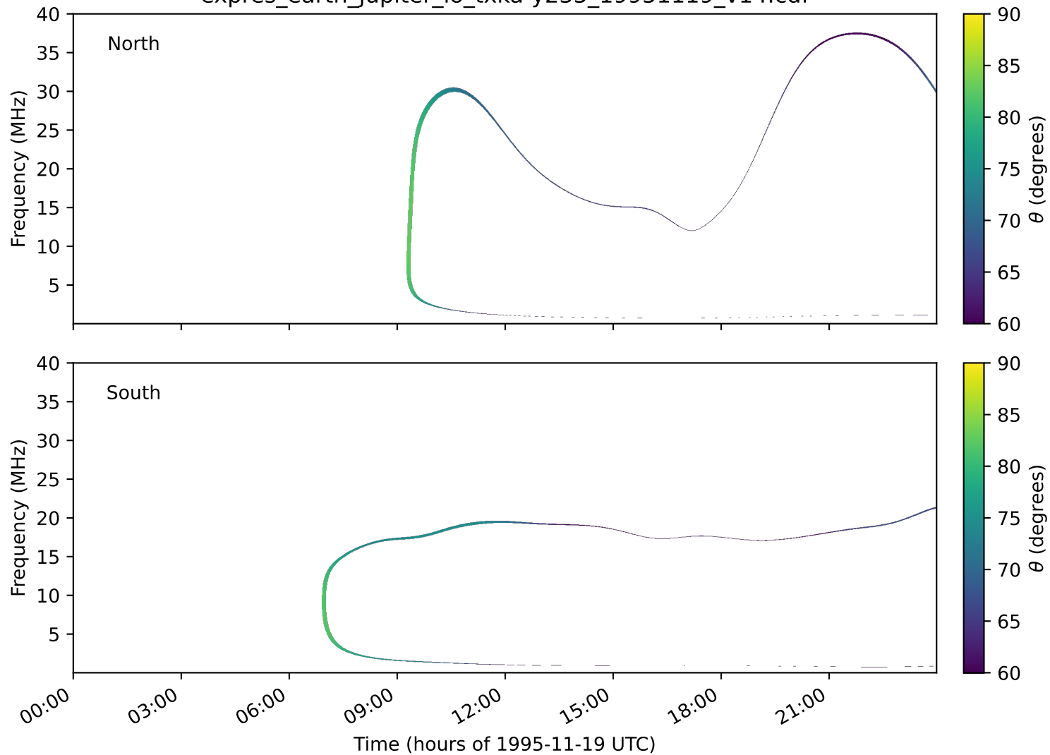
expres_earth_jupiter_io_txka-y235_19951119_v14.cdf
