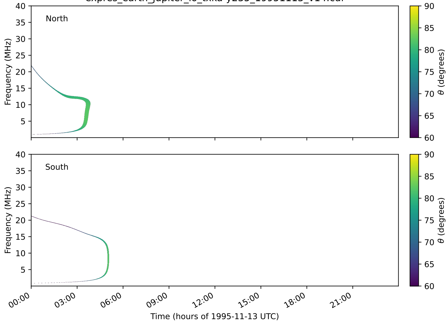
expres_earth_jupiter_io_txka-y235_19951113_v14.cdf
