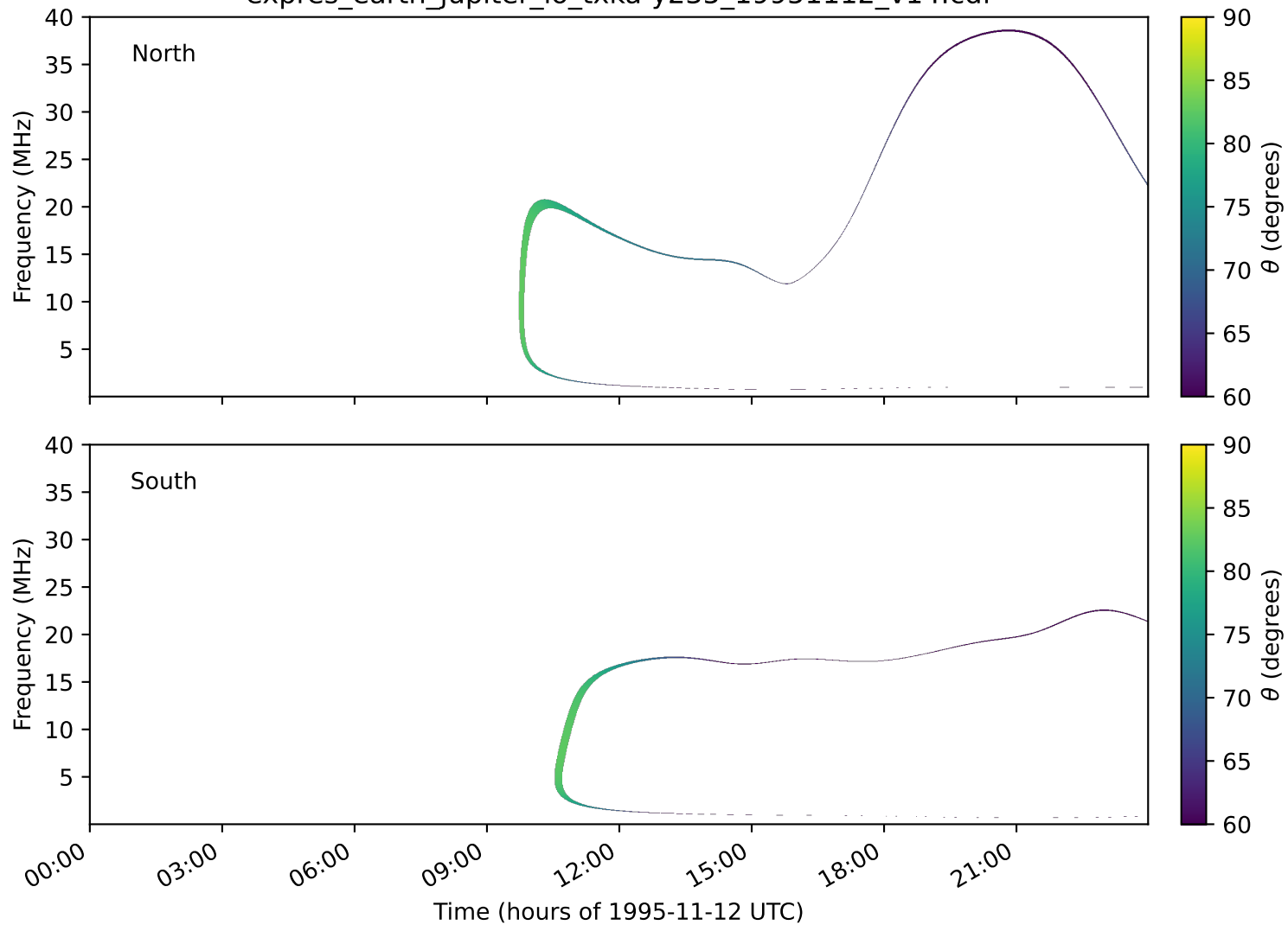
expres_earth_jupiter_io_txka-y235_19951112_v14.cdf
