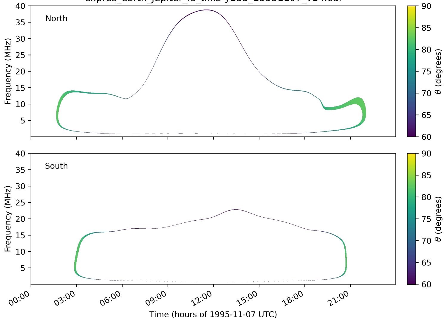
expres_earth_jupiter_io_txka-y235_19951107_v14.cdf
