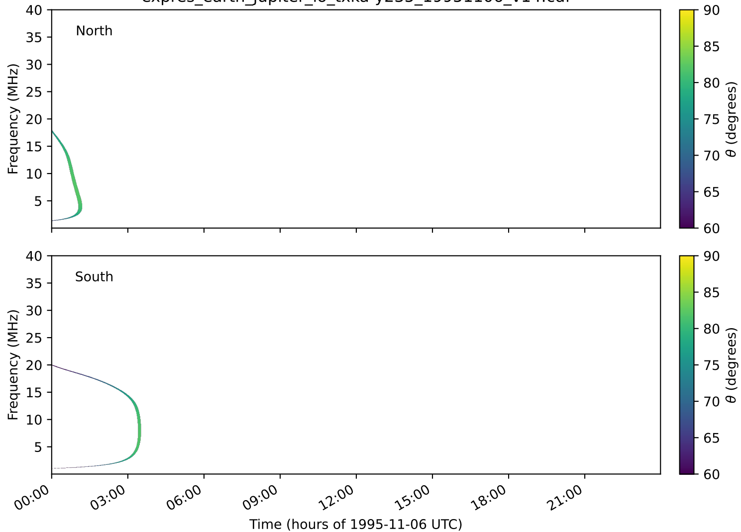
expres_earth_jupiter_io_txka-y235_19951106_v14.cdf
