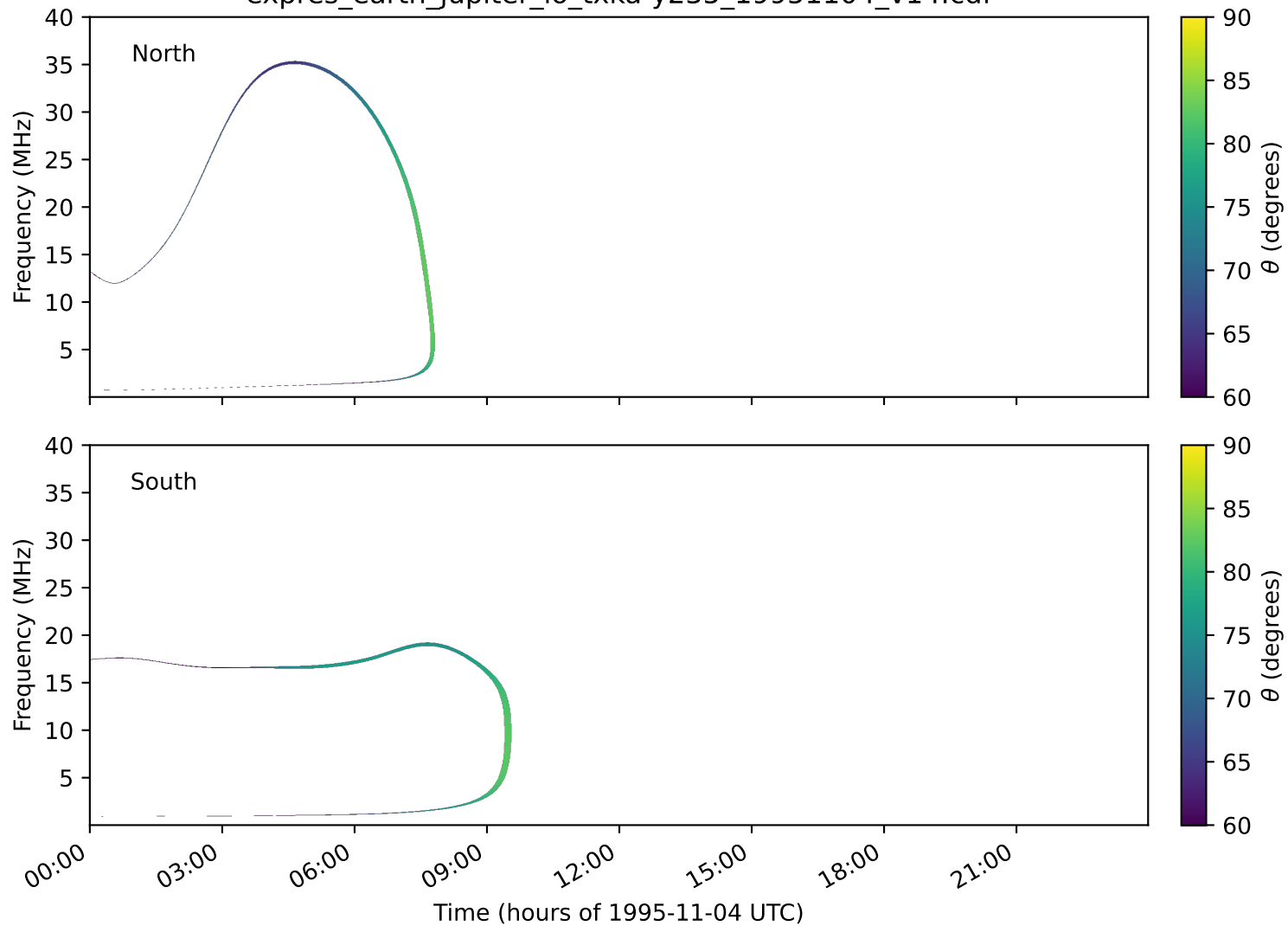
expres_earth_jupiter_io_txka-y235_19951104_v14.cdf
