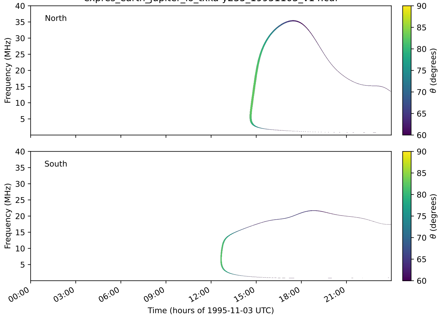
expres_earth_jupiter_io_txka-y235_19951103_v14.cdf
