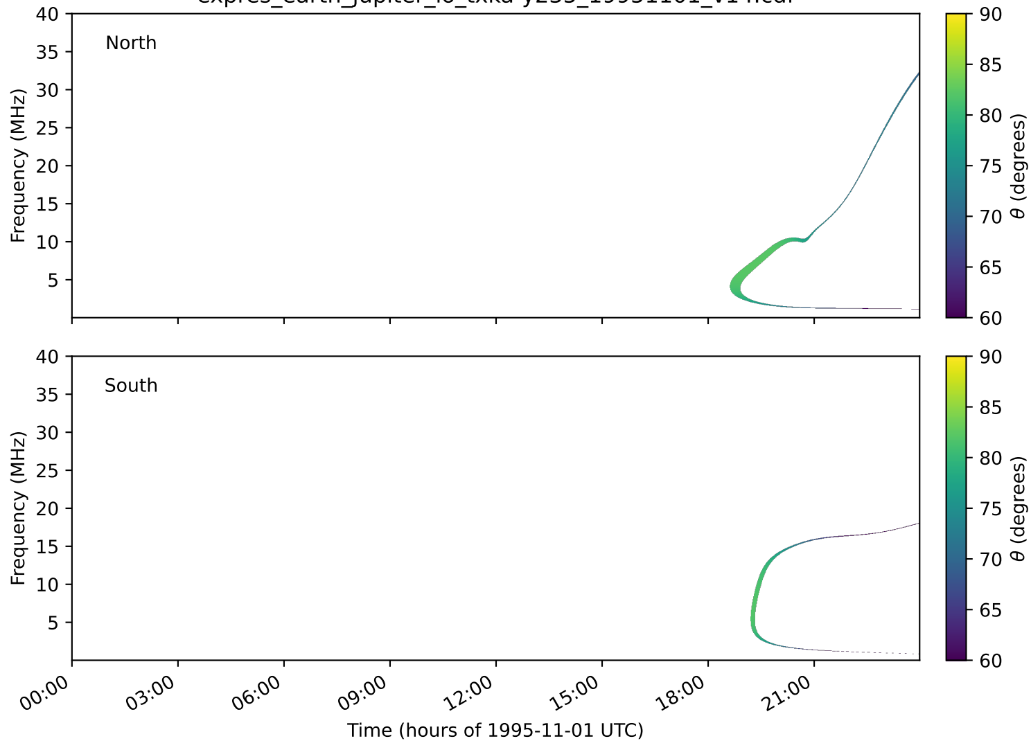
expres_earth_jupiter_io_txka-y235_19951101_v14.cdf
